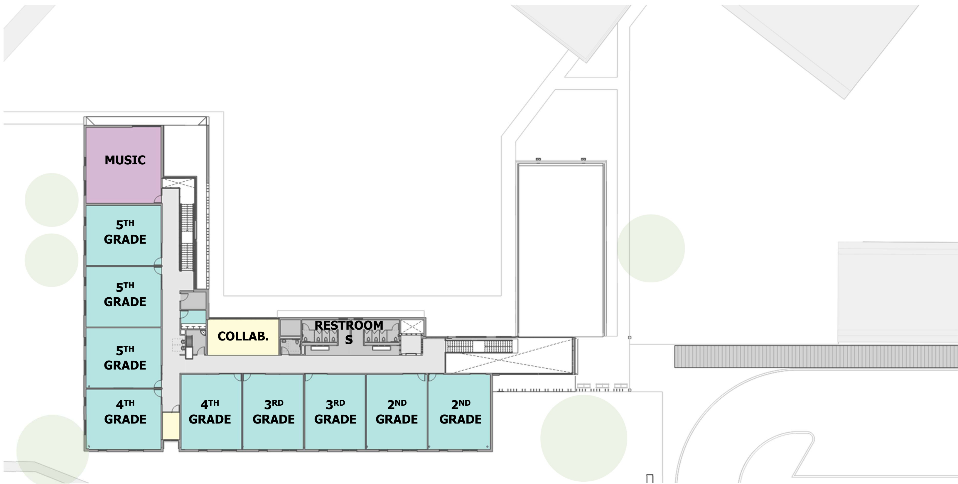
LEVEL 2 FLOOR PLAN 11,602 sqft
