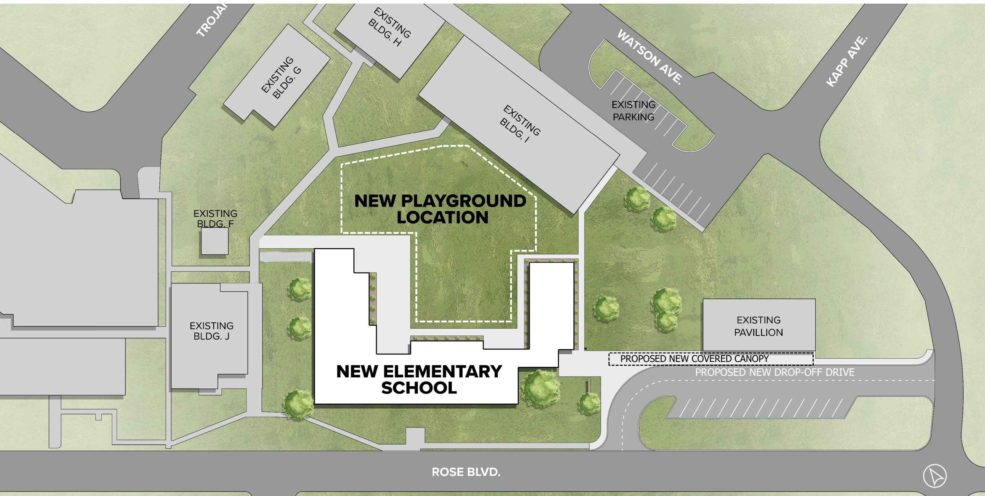
SITE PLAN
